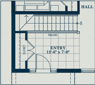
With finished lower level option elev. A & B
