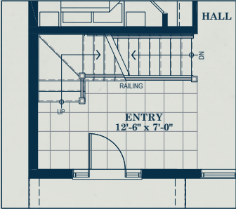
With finished lower level option elev. A & B with Loft
