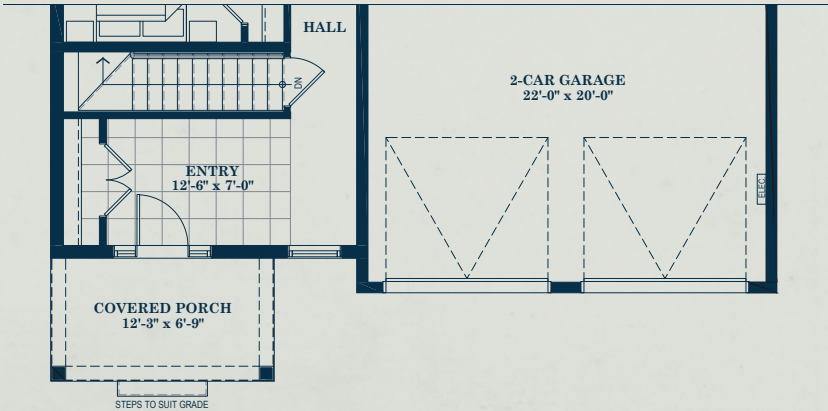
Elevation B Main Level, 1,729 sq ft
