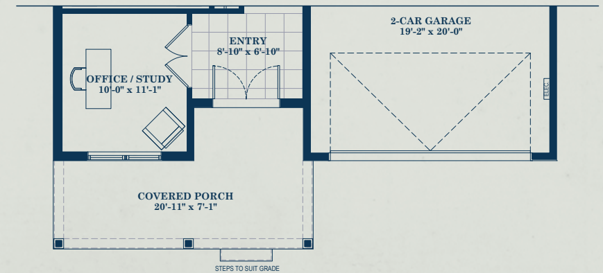
Elevation B Main Level, 1,742 sq ft
